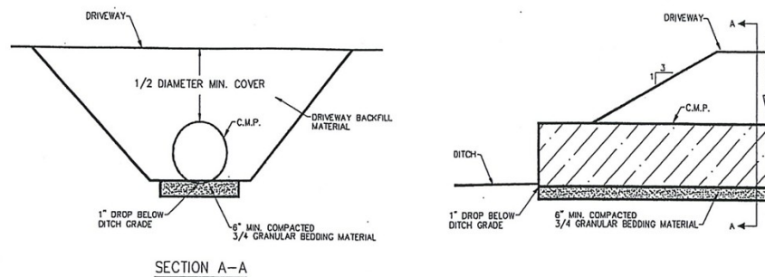
TYPICAL CULVERT INSTALLATION
