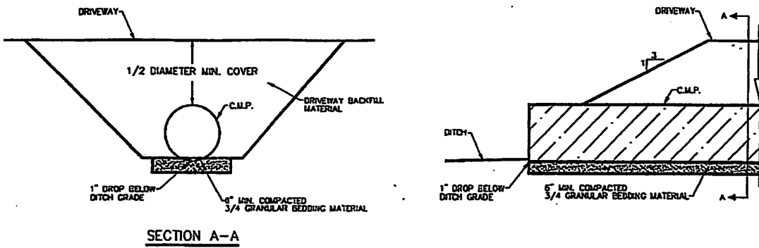
TYPICAL CULVERT INSTALLATION
